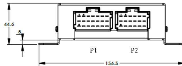
Figure 6: Connector Appearance
