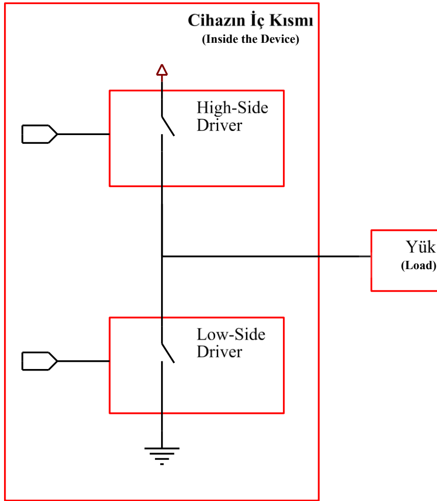
Figure 12: Typical “Half-Bridge” Output Mount connection
