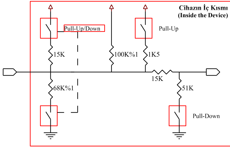
Figure 10: oMux 11x12S Analog Inputs Configuration
