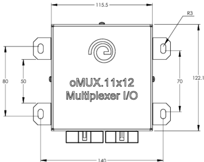
Figure 14: 11x12S oMux Technical Drawing Image
