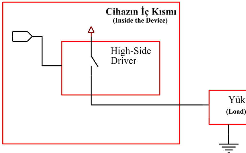
Figure 11: Typical “High-Side” Outlet Mounting connection.
