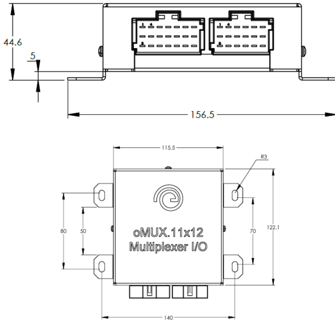
Figure 16: oMux 11x12S dimensions for mounting
