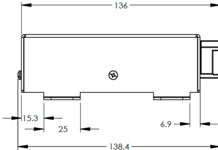
Figure 15: 11x12S oMux Technical Drawing Image
